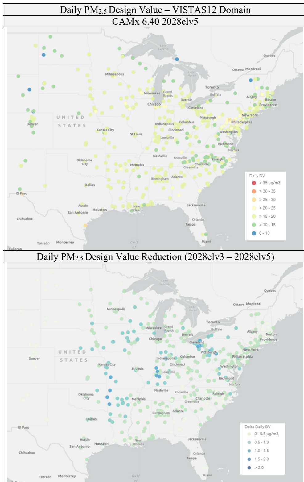
Figure 4-18. Comparison of Daily PM 2.5 Design Values (µg/m 3 ) for CAMx 6.40 2028elv5 and 2028elv3 Simulations
