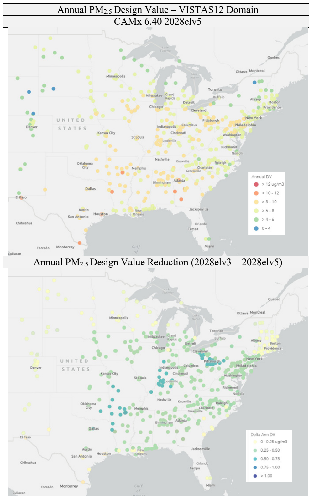
Figure 4-16. Comparison of Annual PM 2.5 Design Values ( \mu\text{g}/\text{m}^3 ) for CAMx 6.40 2028elv5 and 2028elv3 Simulations
